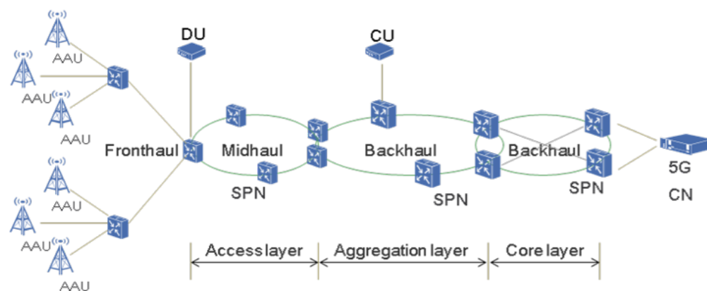
Figure 4-1: Mobile Transport
