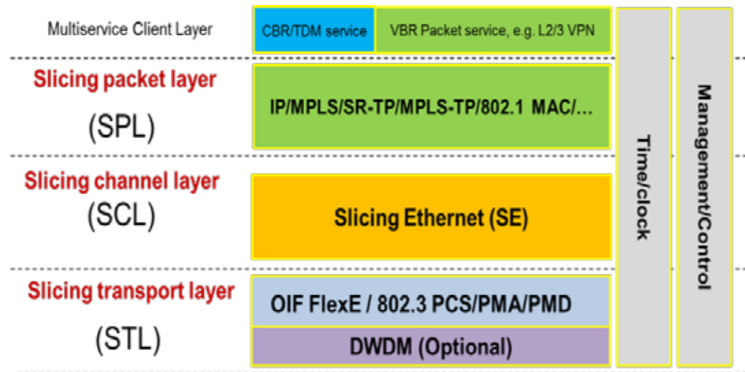
Figure 2-2: Layered SPN network model
