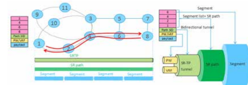
Figure 3-6: SRTP-TE Tunnel
