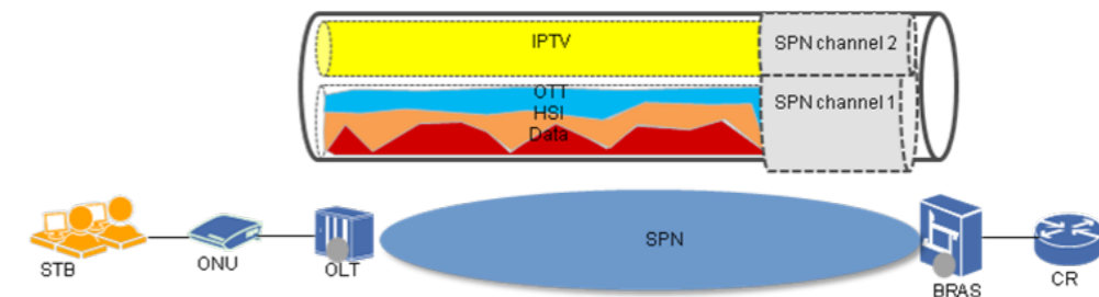
Figure 4-4: SPN-based big video service transport
